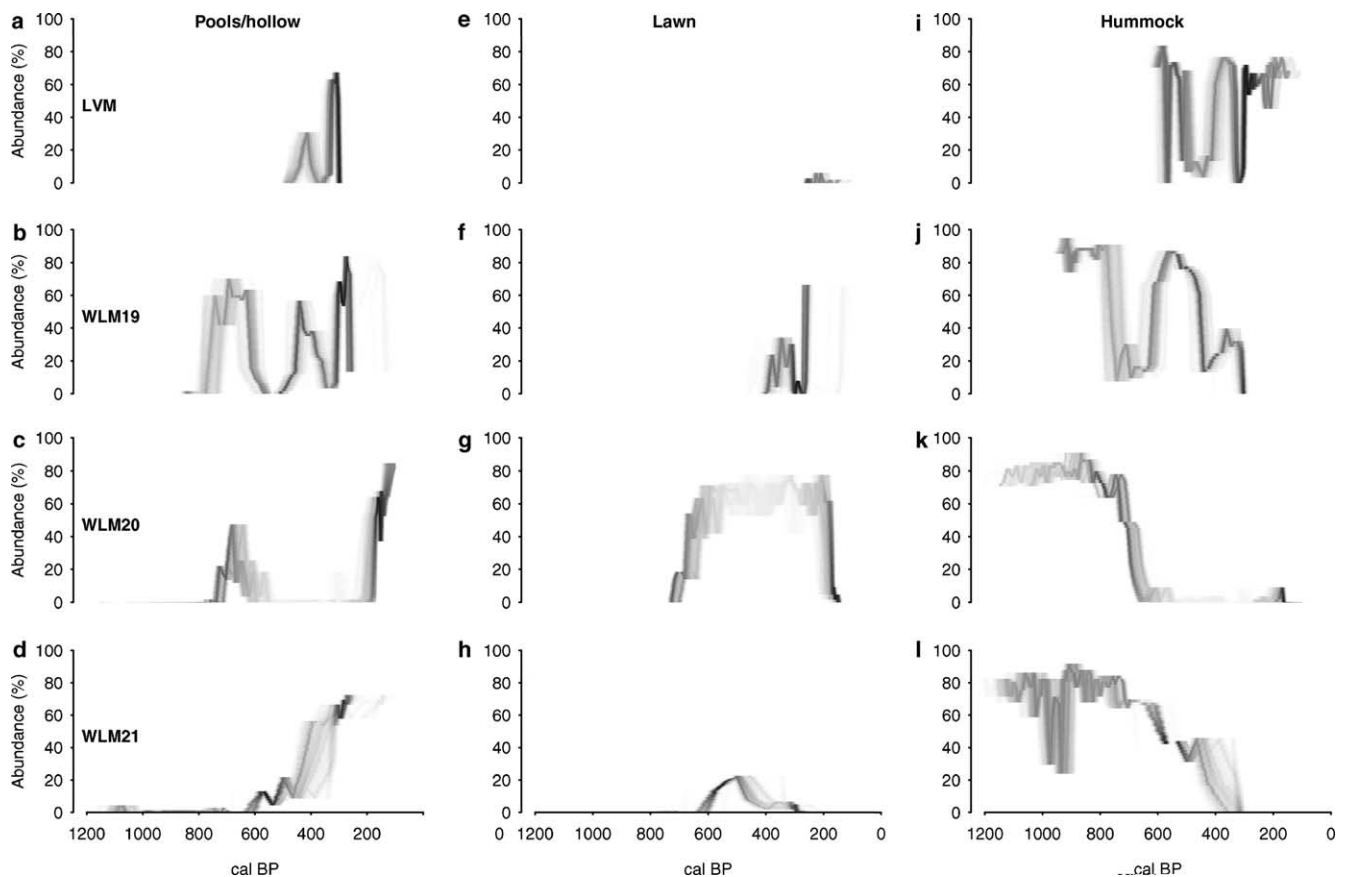
Figure 2 Chronologies of macrofossil-inferred local wetness from core LVM (a,e,i) and replicate cores WLM19 (b,f,j), WLM20 (c,g,k) and WLM21 (d,h,l) (Mauquoy et al. , 2002a,b). a–d, combined abundances of pool/hollow species ( Sphagnum cuspidatum , S. Sect. Cuspidata and S. tenellum ), indicating wet conditions; e–h, combined abundances of lawn species ( S. magellanicum and S. papillosum ), indicating intermediate moisture; i–l, combined abundances of hummock species ( S. imbricatum and S. capillifolium ), indicating dry conditions
